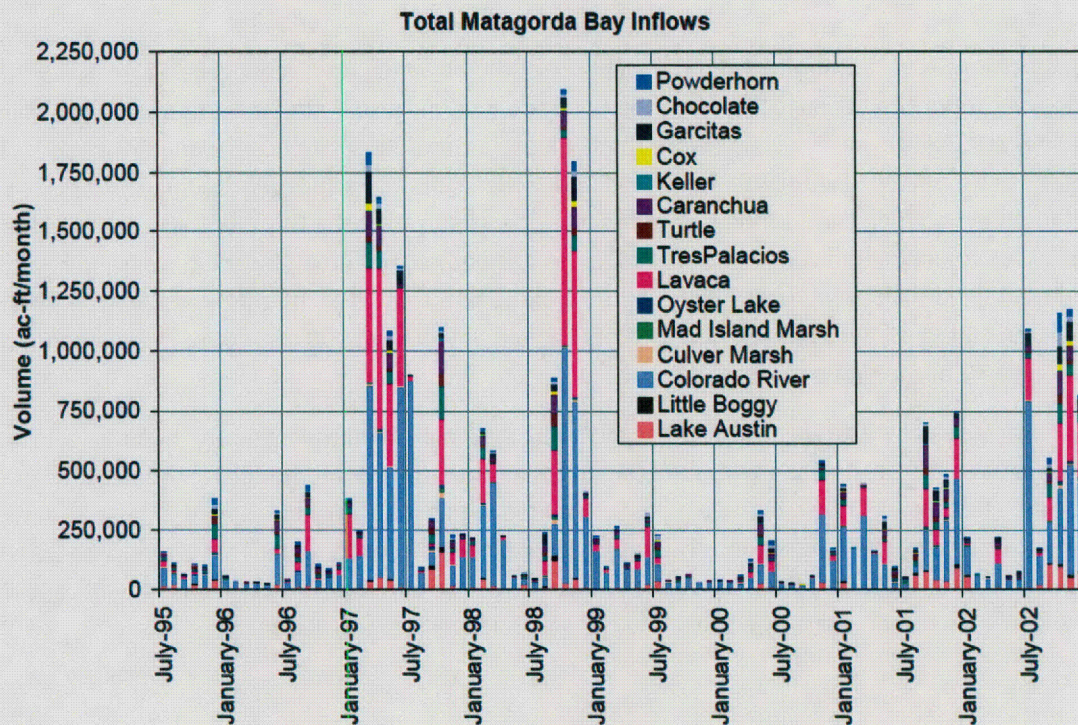
Figure 6. Distribution of monthly inflows to the Matagorda Bay system (MBHE 2007).
