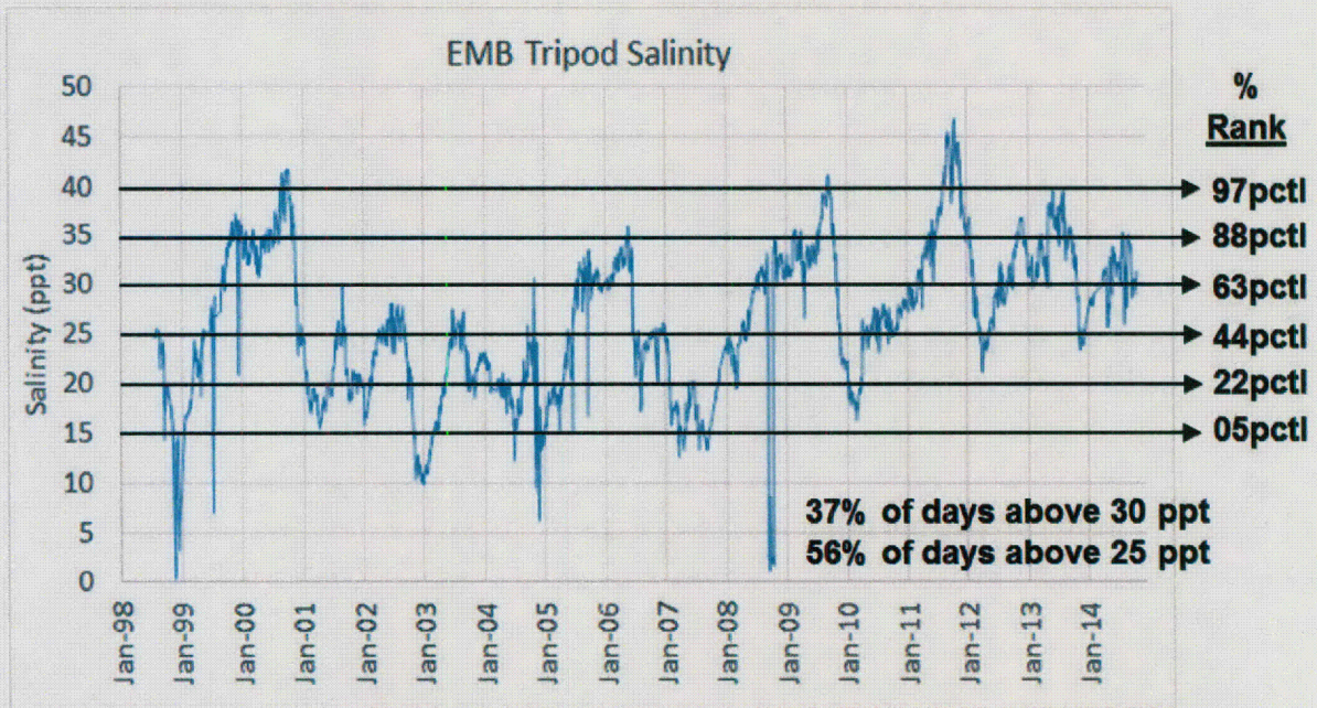
Figure 13. Historical observed salinity data at East Matagorda Bay "Tripod" sonde, with percentile statistics.
