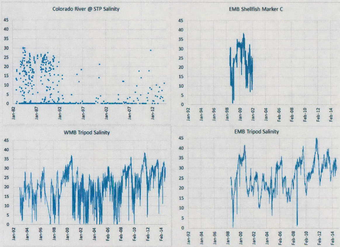
Figure 10. Selected LCRA daily salinity (ppt) sonde data.
