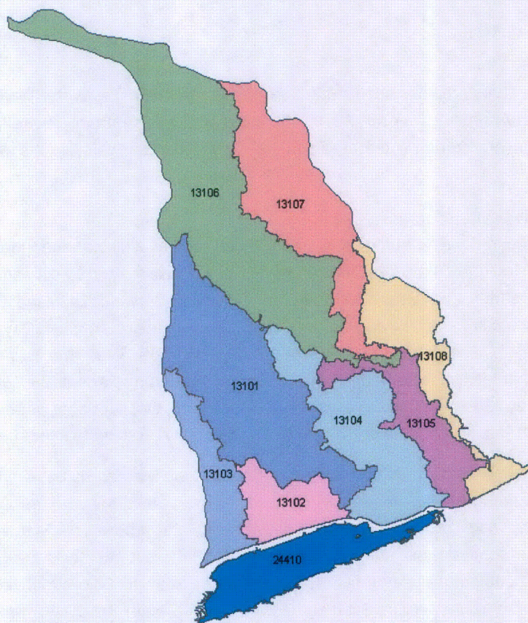
Figure 3. Unengaged watershed delineation used in TxRR to determine unengaged inflows to the East Matagorda Bay System (Shoenbaechler and Guthrie, 2011).
