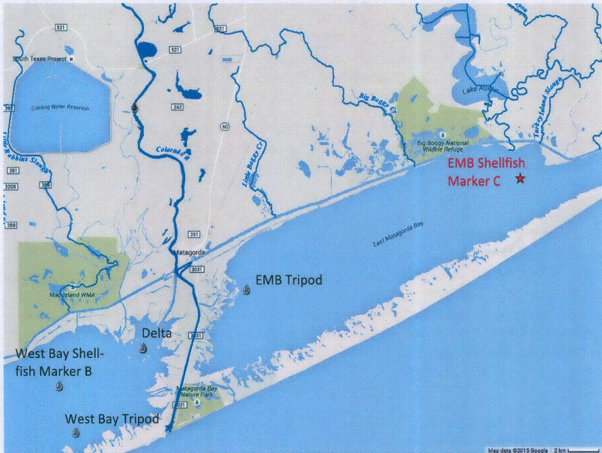
Figure 9. LCRA continuous salinity monitoring locations (data at grey rain drops available online: waterquality.lcra.org ).
