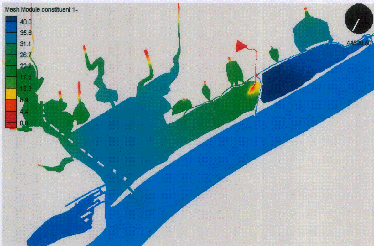
Figure 12. MBHE RMA2/RMA4 Salinity Model year July 2000 (MBHE 2009). Salinity in parts per thousand.
