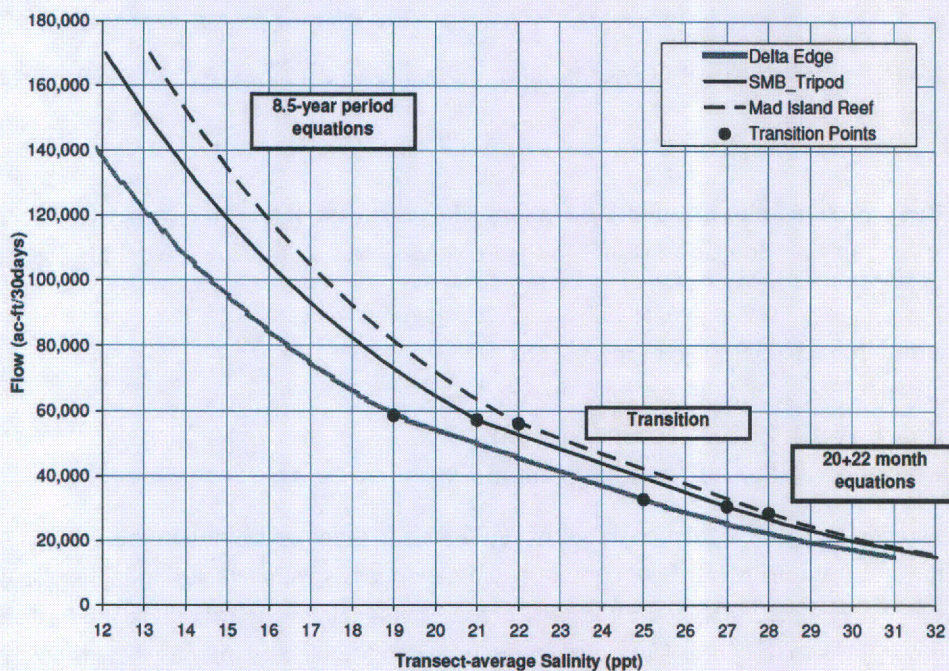
Figure 27. Relationship between inflow and average salinity in Delta area of Matagorda Bay (MBHE 2008).
