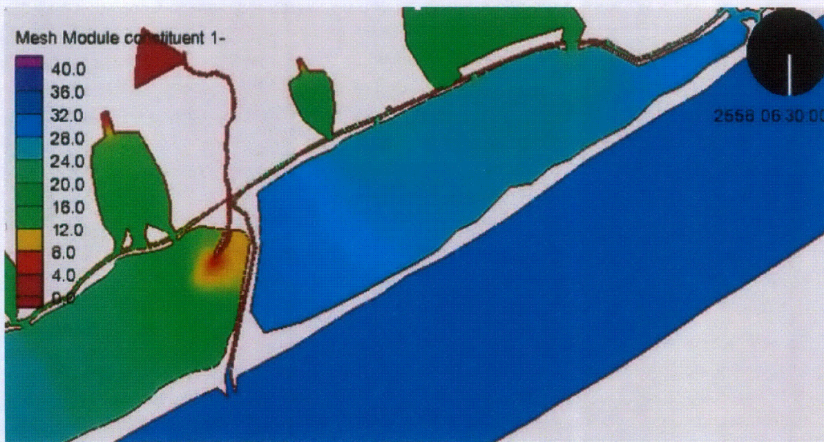
Figure 16. RMA2 salinity prediction at end of June 2002. Salinity in parts per thousand
