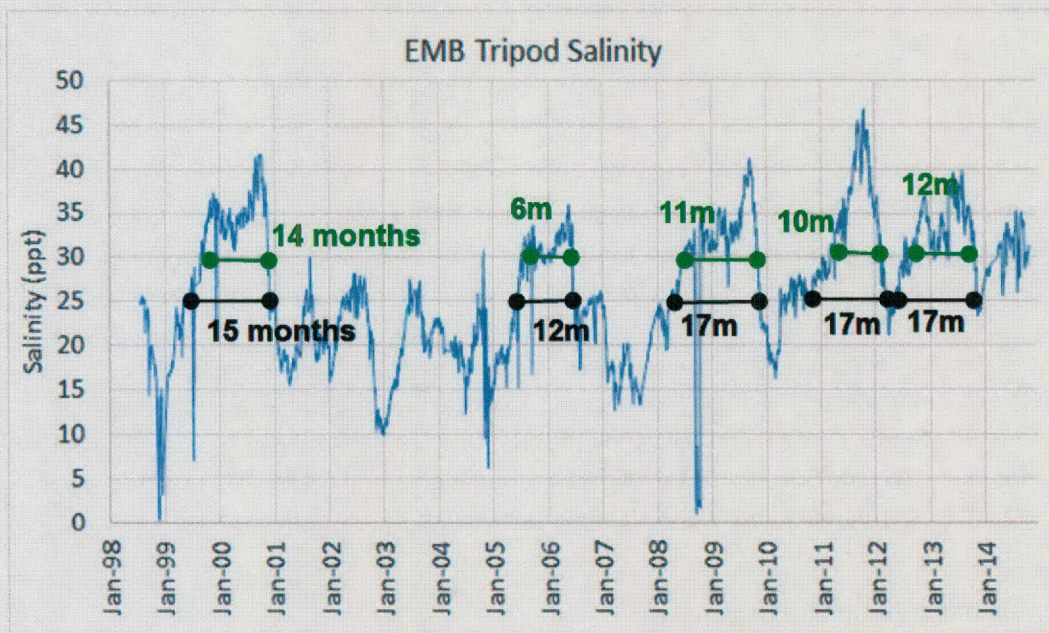
Figure 14. Historical observed salinity data at East Matagorda Bay "Tripod" sonde, with duration of events exceeding 25 ppt and 30 ppt.
