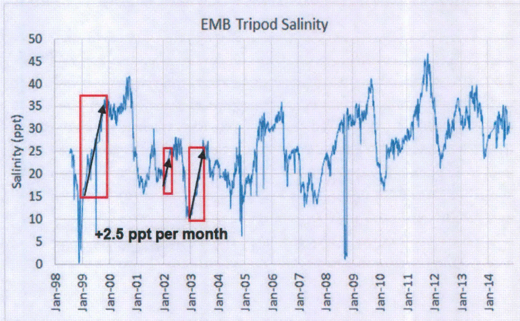
Figure 15. Historical observed salinity data at East Matagorda Bay “Tripod” sonde, with illustration of rebound following inflow freshening events.
