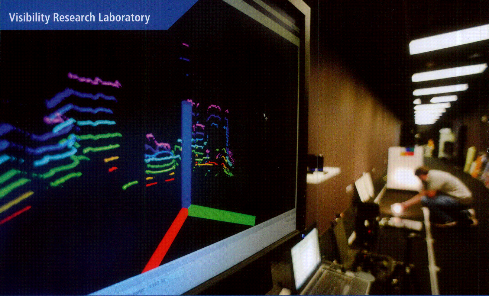
Evaluating the use of lasers to assess retroreflective infrastructure condition.
