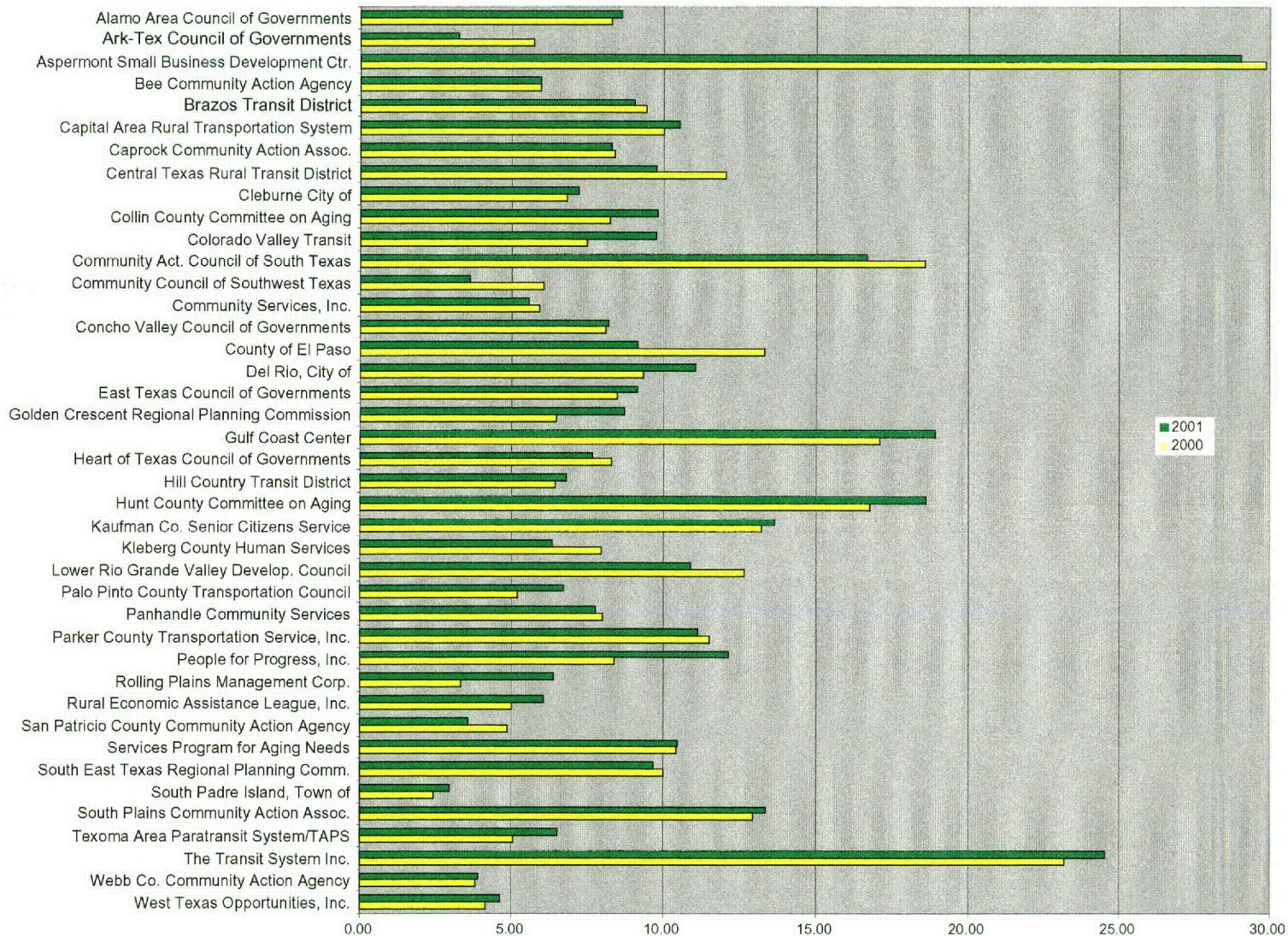
Figure 10: Nonurbanized Area Programs (5311) Cost per Passenger Trip
