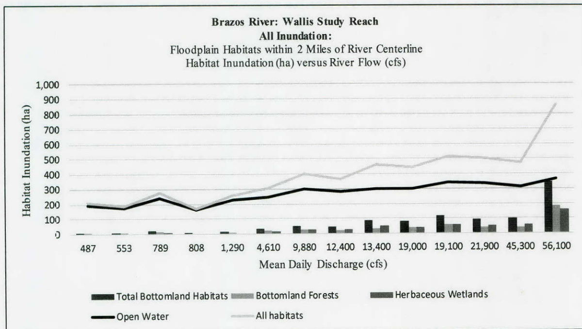
Figure 6 All Inundation: Wallis Study Reach (graph) Habitat Inundation versus Mean Daily Discharge
