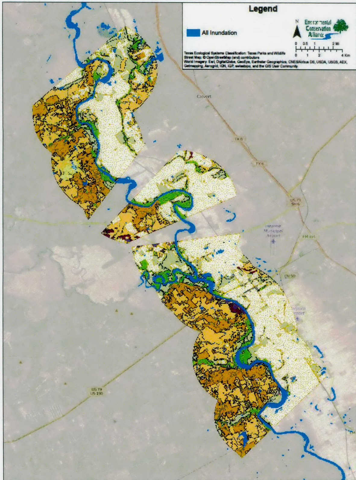
Figure 9.5 All Inundation Map: Wallis Study Reach 01/19/92 Inundation Event: 56,100 cfs
