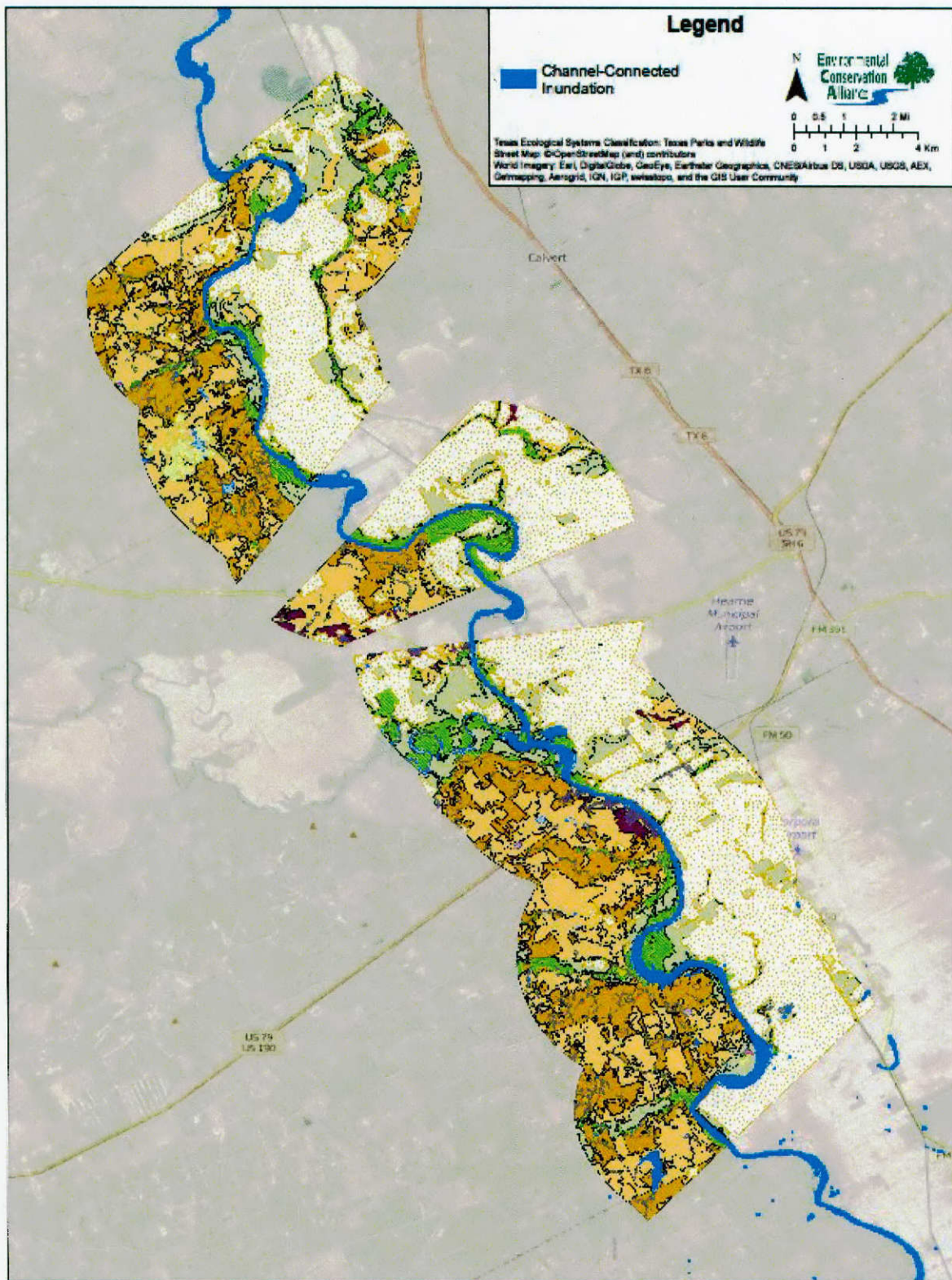
Figure 9.2 Channel-Connected Inundation Map: Wallis Study Reach 01/19/92 Inundation Event: 56,100 cfs
