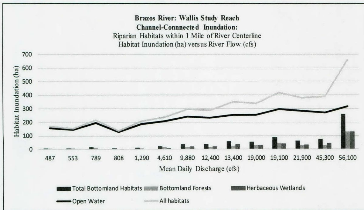
Figure 5. Channel-Connected Inundation: Wallis Study Reach (graph) Habitat Inundation versus Mean Daily Discharge
