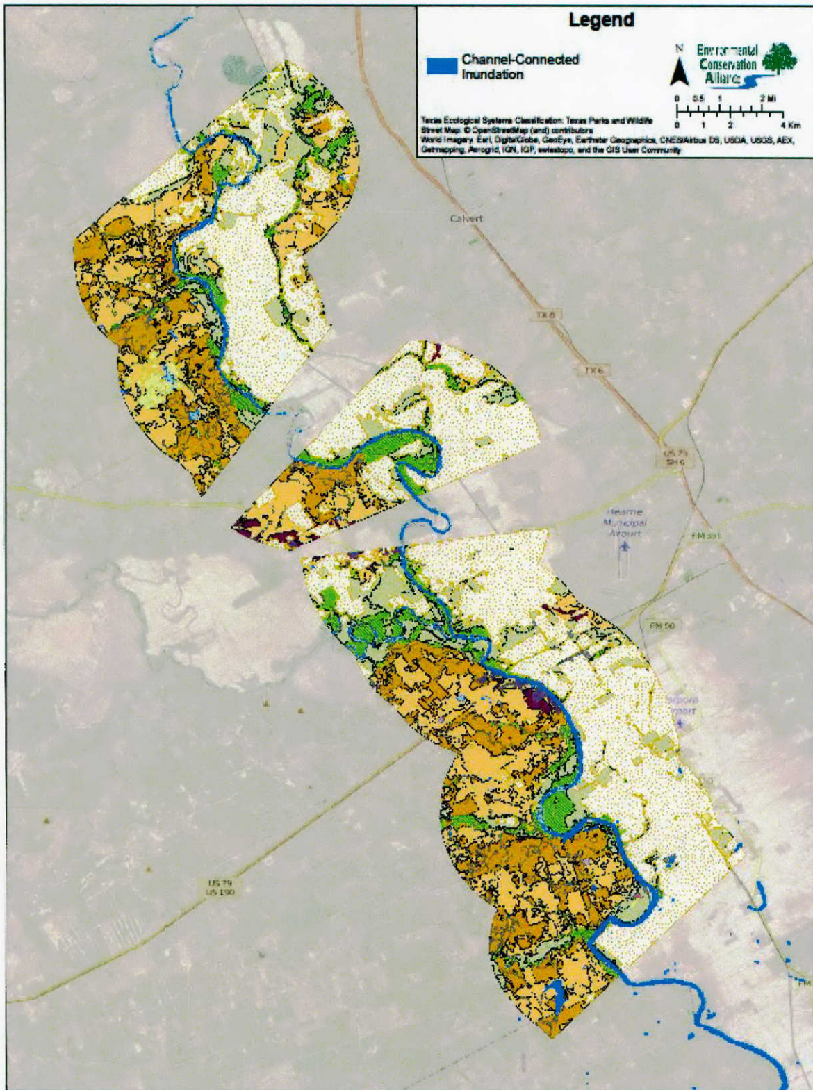
Figure 9.4 Channel-Connected Inundation Map: Wallis Study Reach 02/02/09 Inundation Event: 487 cfs
