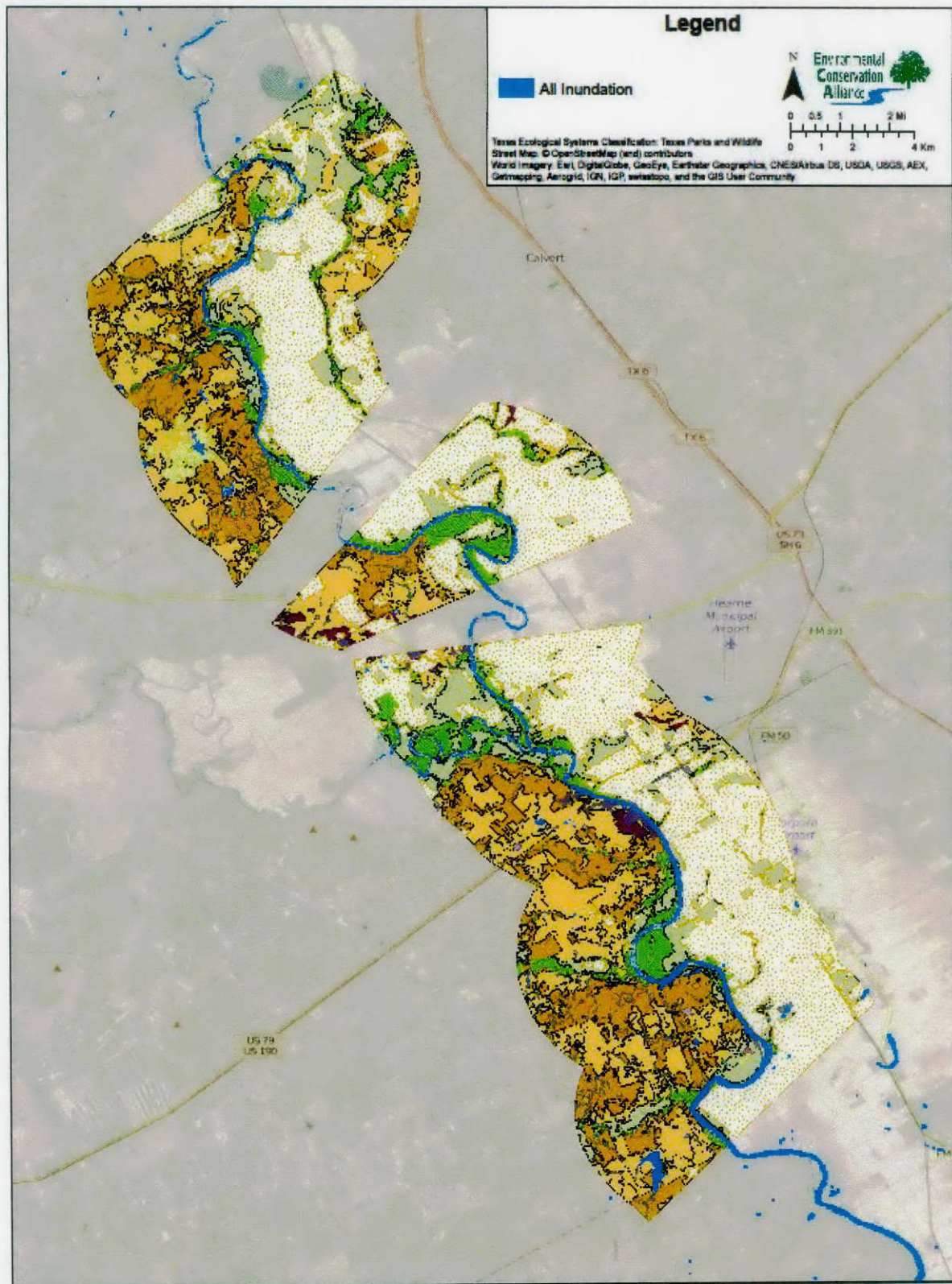
Figure 9.7 All Inundation Map: Wallis Study Reach 02/02/09 Inundation Event: 487 cfs
