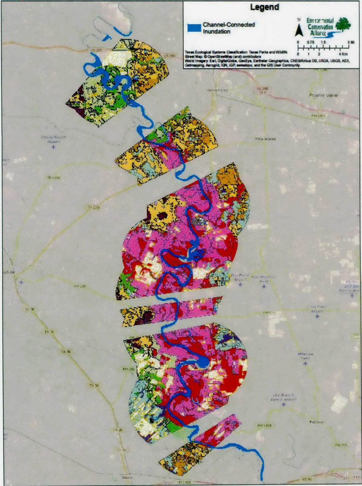
Figure 10.2 Channel-Connected Inundation Map: San Felipe Study Reach 03/07/92 Inundation Event: 71,000 cfs
