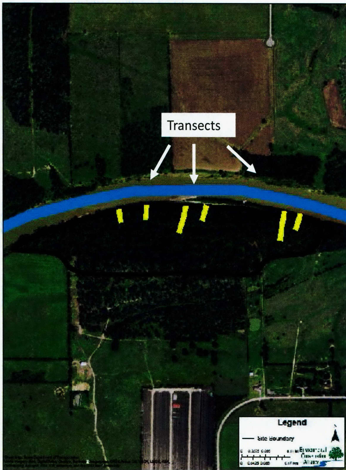
Figure 4.2 Wallis Study Site: Transect Locations
