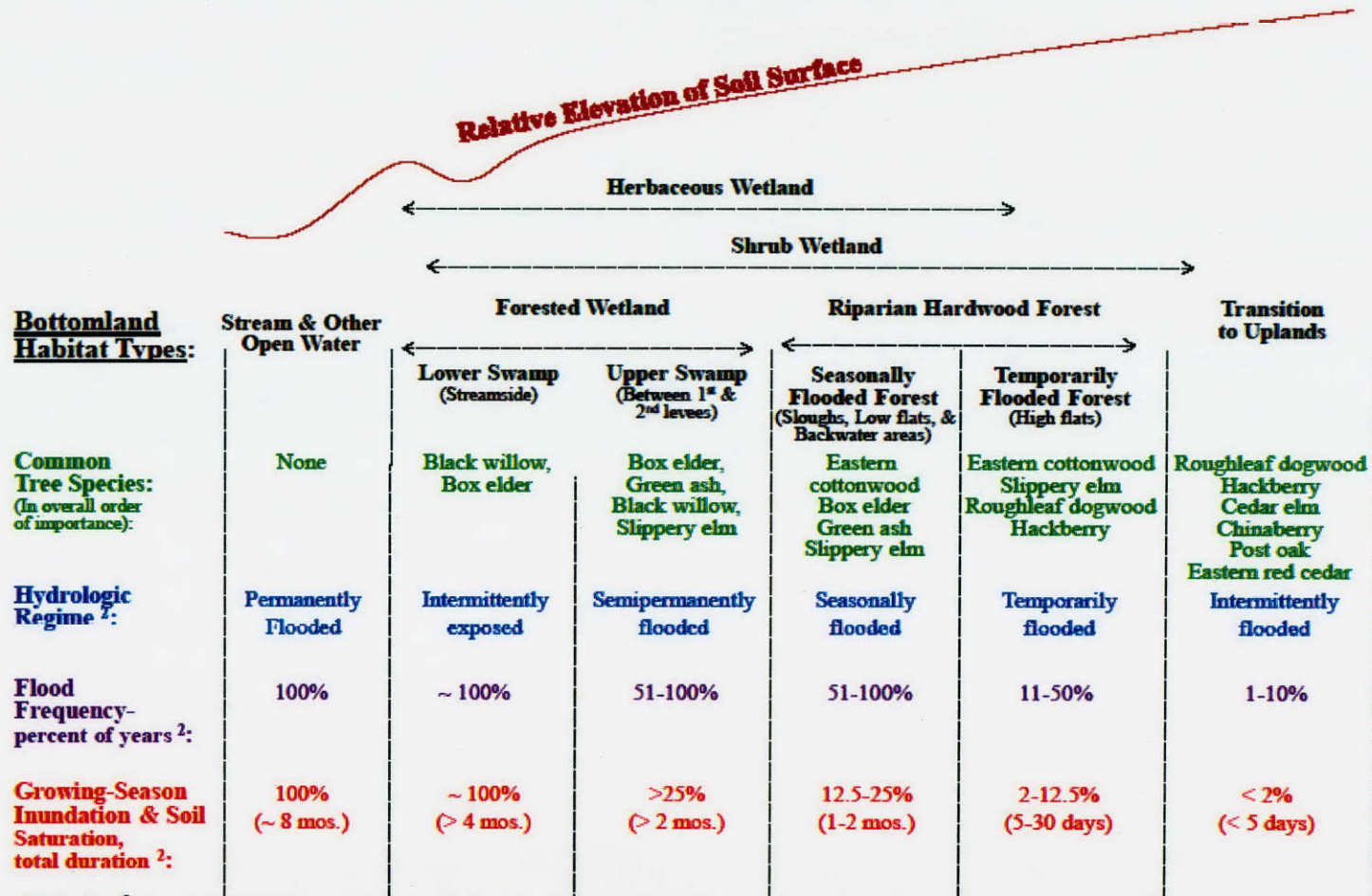
Figure 1 Riparian Habitats in Lower Brazos River Study Areas: Landscape Context, Tree Species, and Hydrology
