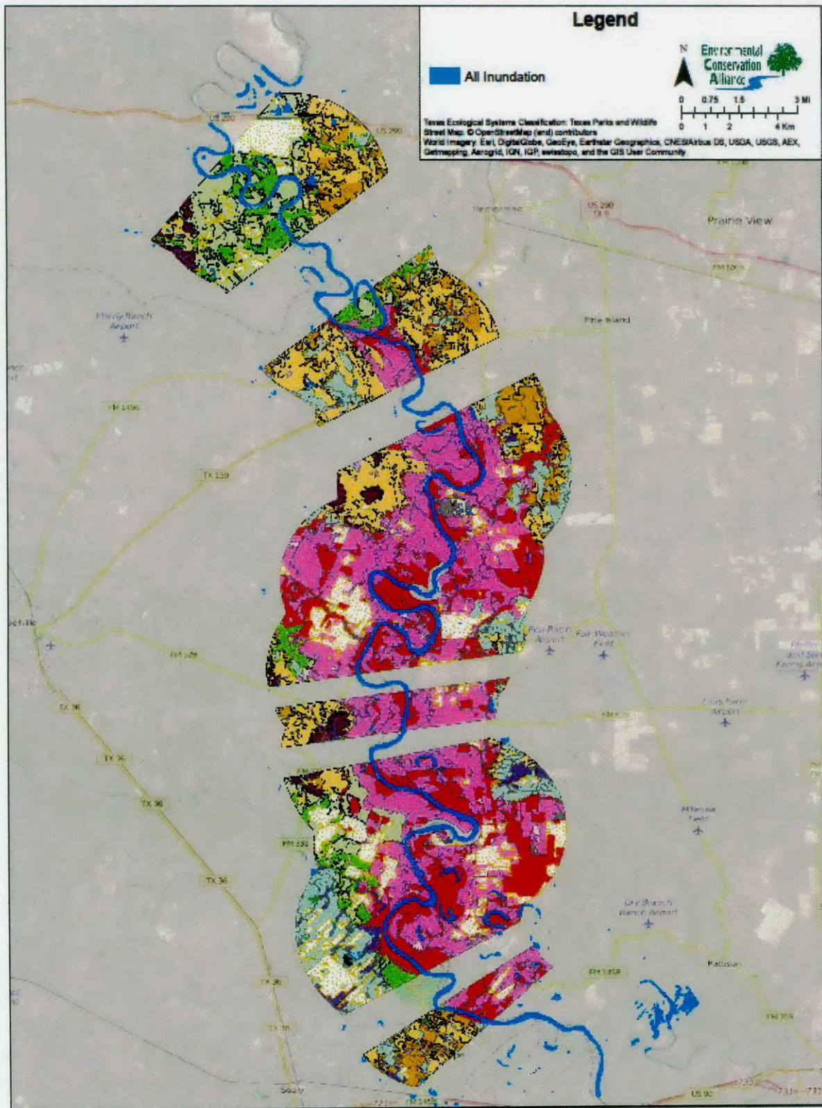
Figure 10.6 All Inundation Map: San Felipe Study Reach 02/25/94 Inundation Event: 19,200 cfs
