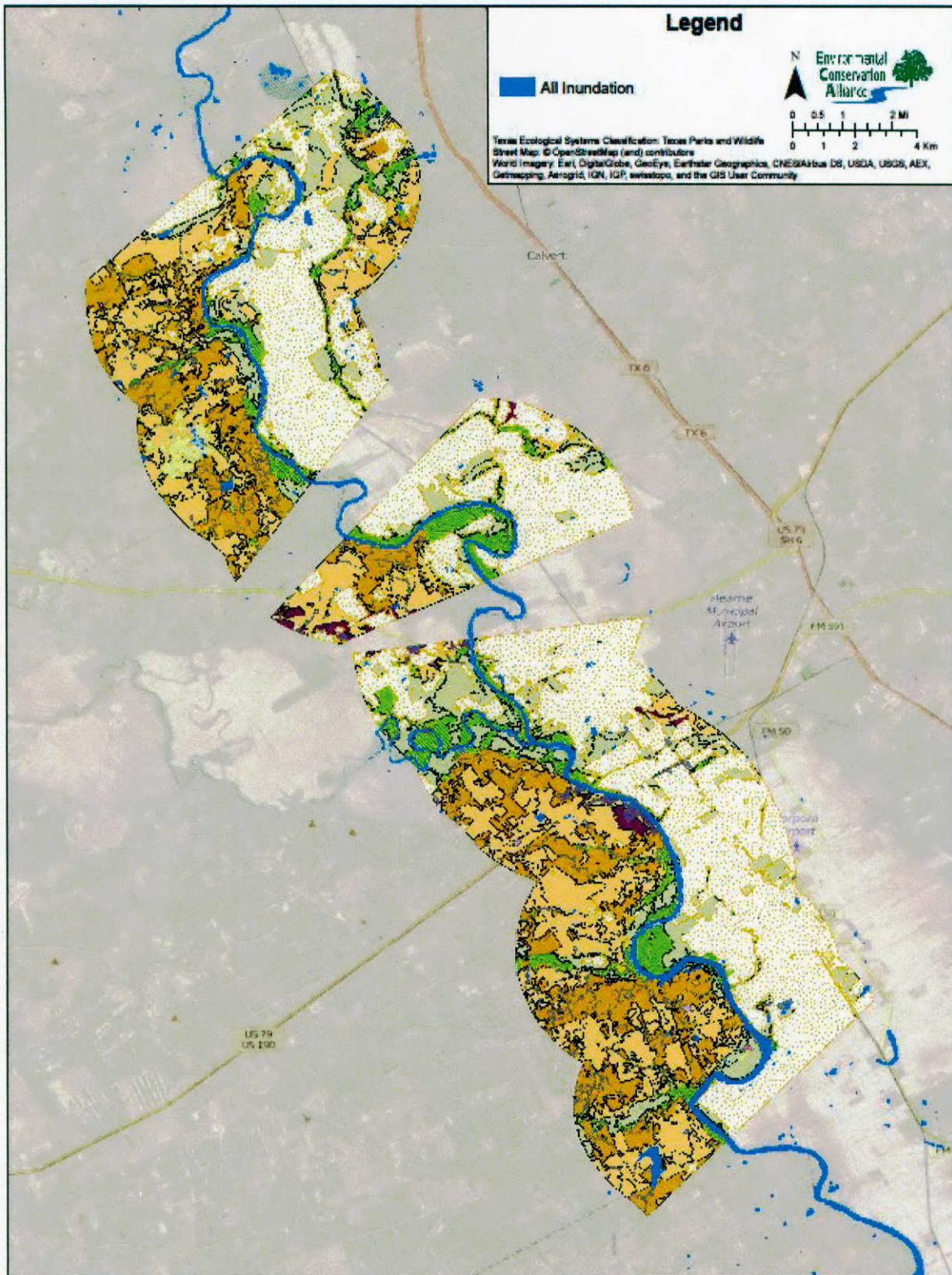
Figure 9.6 All Inundation Map: Wallis Study Reach 01/19/01 Inundation Event: 13,400 cfs
