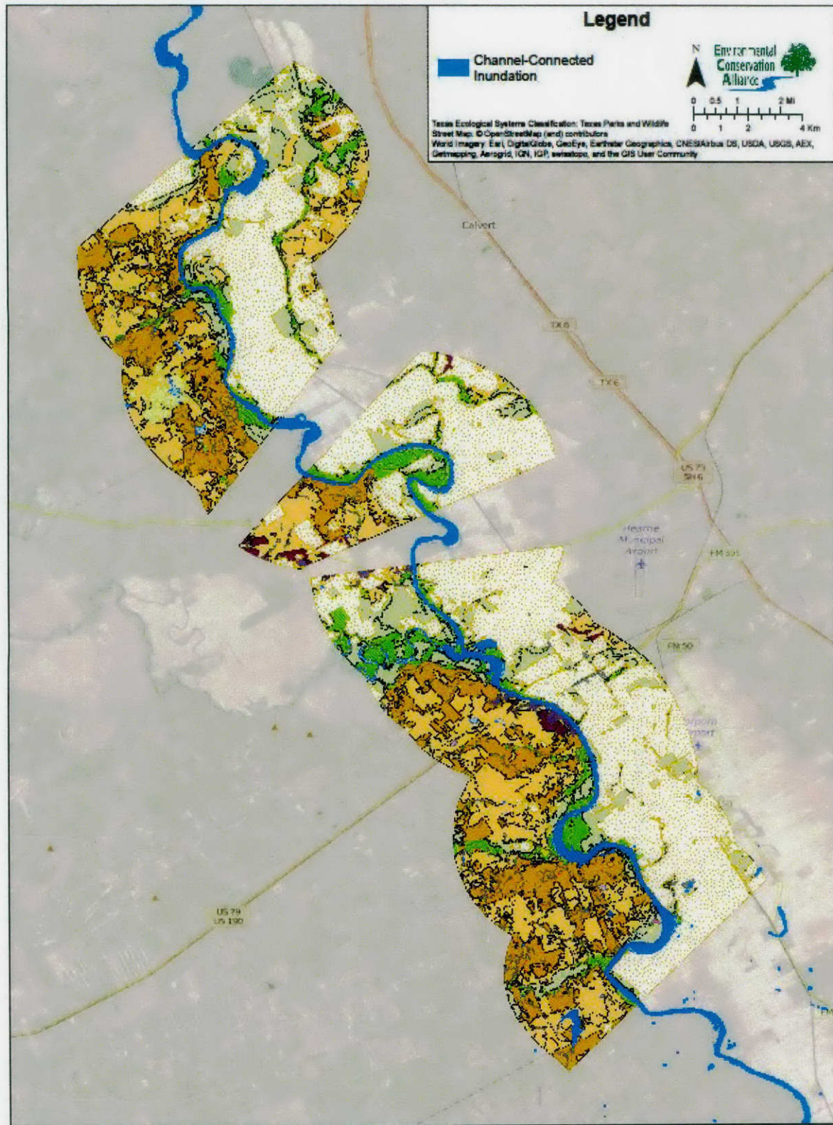
Figure 9.3 Channel-Connected Inundation Map: Wallis Study Reach 01/19/01 Inundation Event: 13,400 cfs
