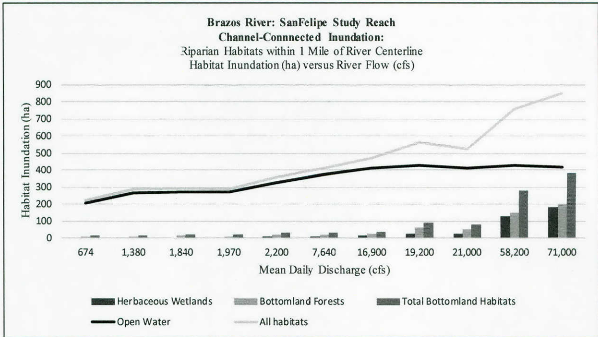
Figure 8 All Inundation: San Felipe Study Reach (graph) Habitat Inundation versus Mean Daily Discharge
