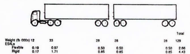
Figure 3.2: ESAL values for various trucks
