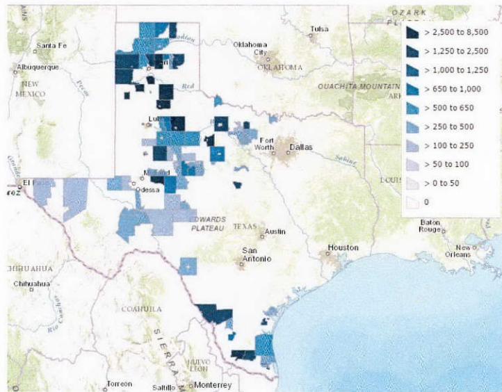
Figure 1.6: Number of turbines installed in Texas for the year 2025
