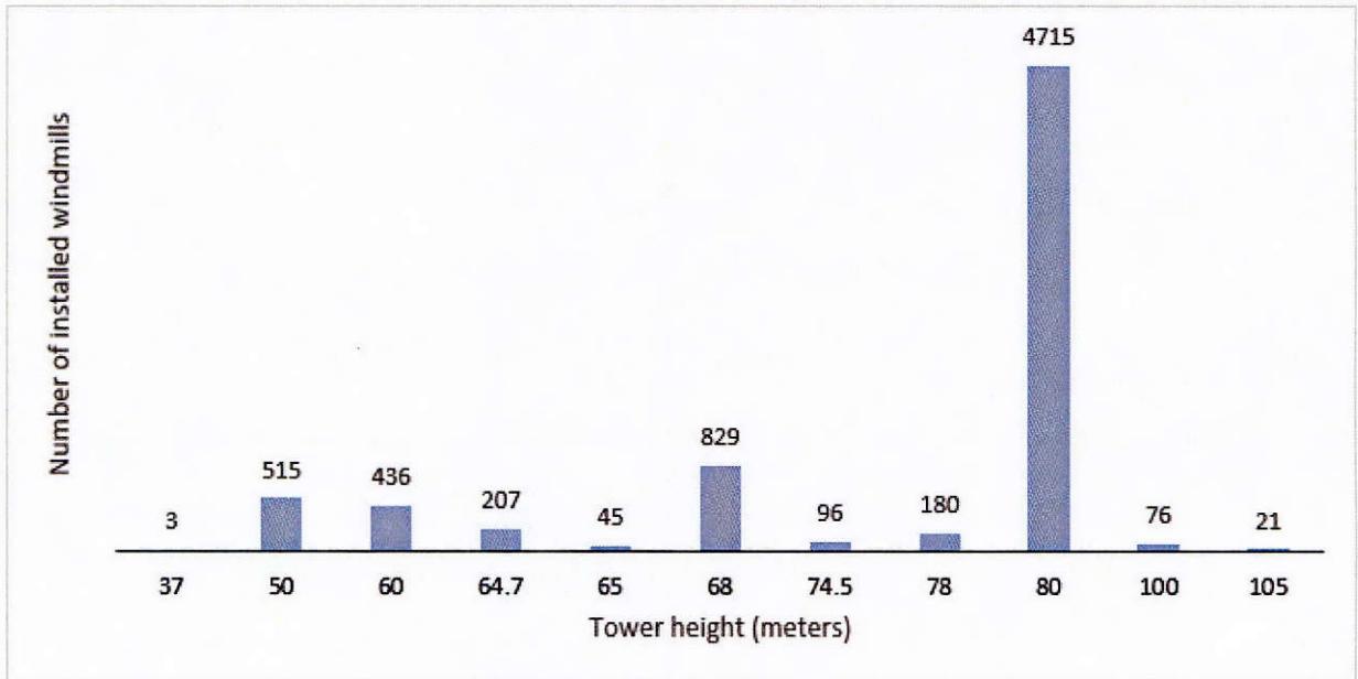
Figure 2.4: Number of installed windmills by tower height
