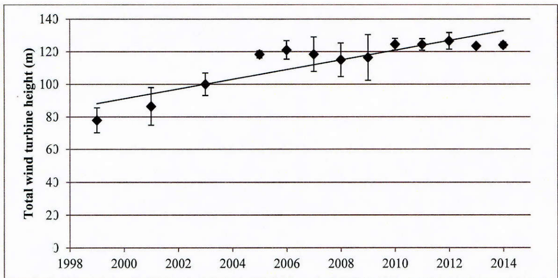
Figure 2.9: Evolution of wind turbine total heights
