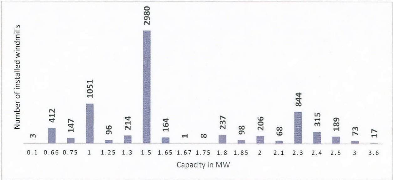
Figure 2.3: Windmill installations in terms of power-generating capacity
