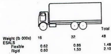
(b) Four-Axle Single-Unit Truck
