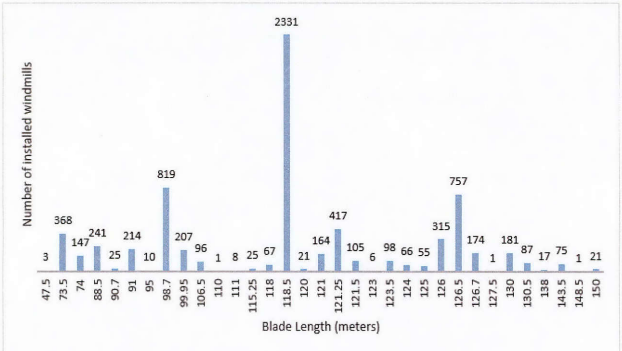
Figure 2.5: Number of windmills installed by blade length
