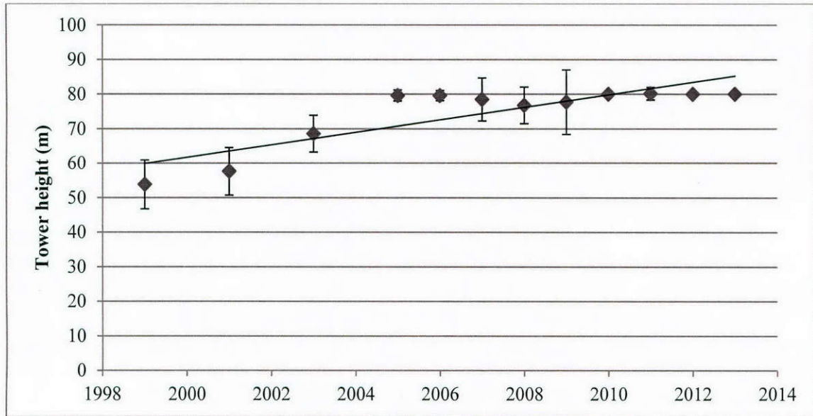
Figure 2.10: Evolution of tower heights
