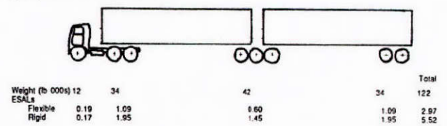
(g) Eight-Axle B-Train Double (3-S3-2)
