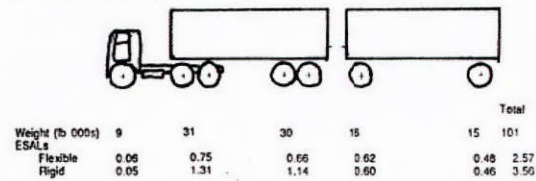
(g) Eight-Axle B-Train Double (3-S3-2)
