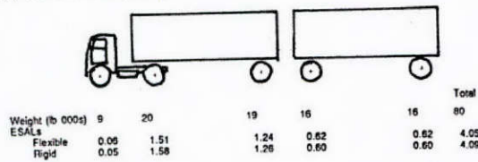
Figure 3.2: ESAL values for various trucks
