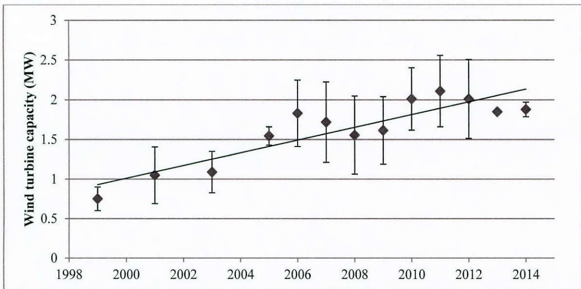
Figure 2.7: Evolution of turbine capacities installed in Texas
