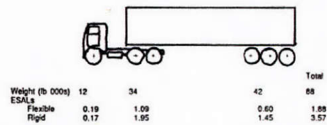
(f) Seven-Axle Double (3-S2-2)
